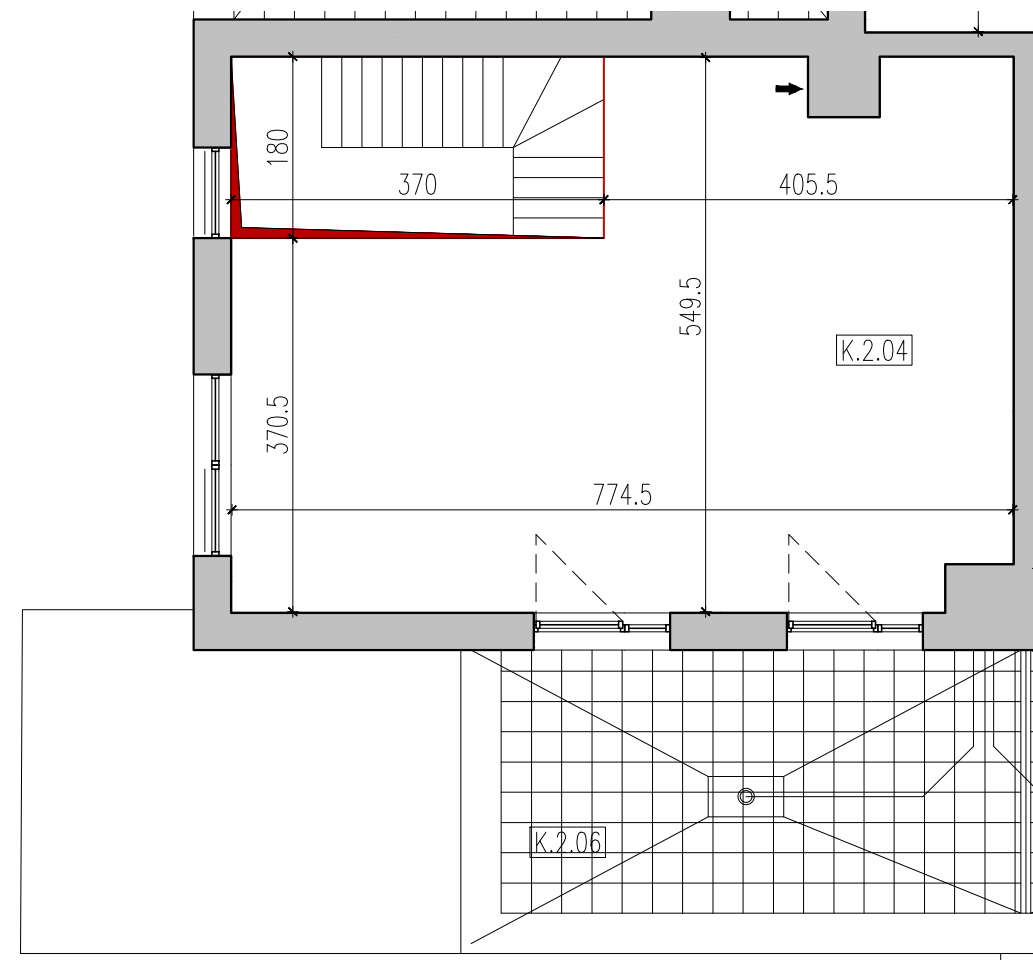
ANTRESOLA
